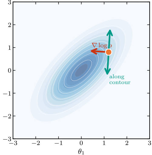
HMC: gradient reveals which directions explore
