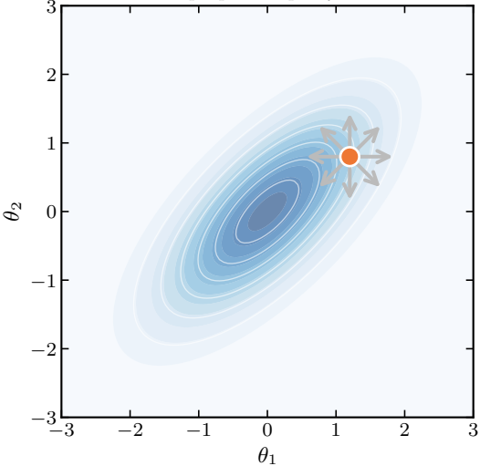
Random walk: proposes equally in all directions
