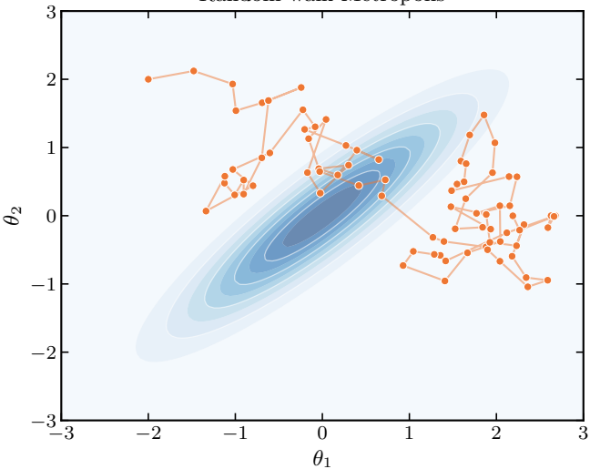
Random walk Metropolis
