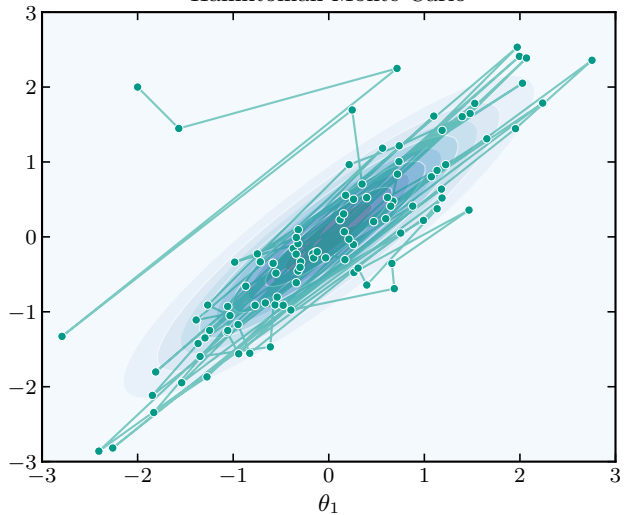
Hamiltonian Monte Carlo
