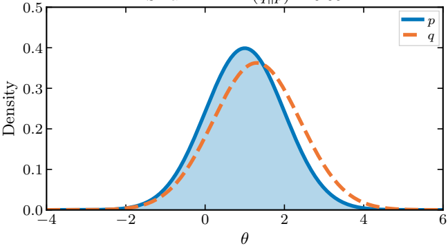
Small KL: \text{KL}(q||p) = 0.05
