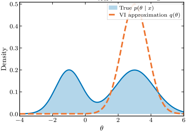
VI minimizes \text{KL}(q||p) : mode-seeking
