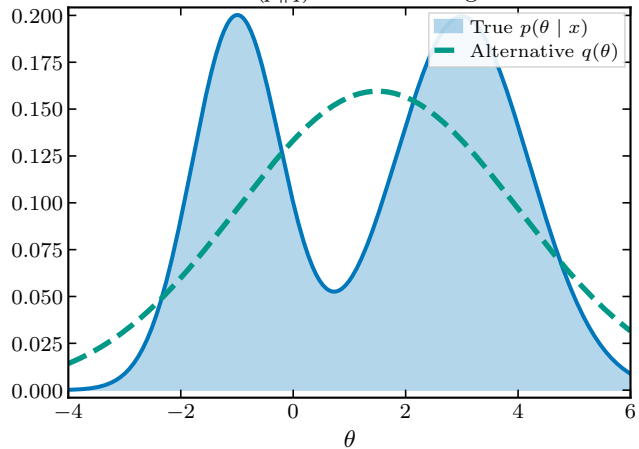
\text{KL}(p||q) : mass-covering
