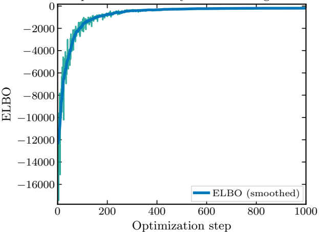
VI optimization on Bayesian linear regression
