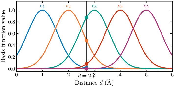
(a) Radial basis functions
