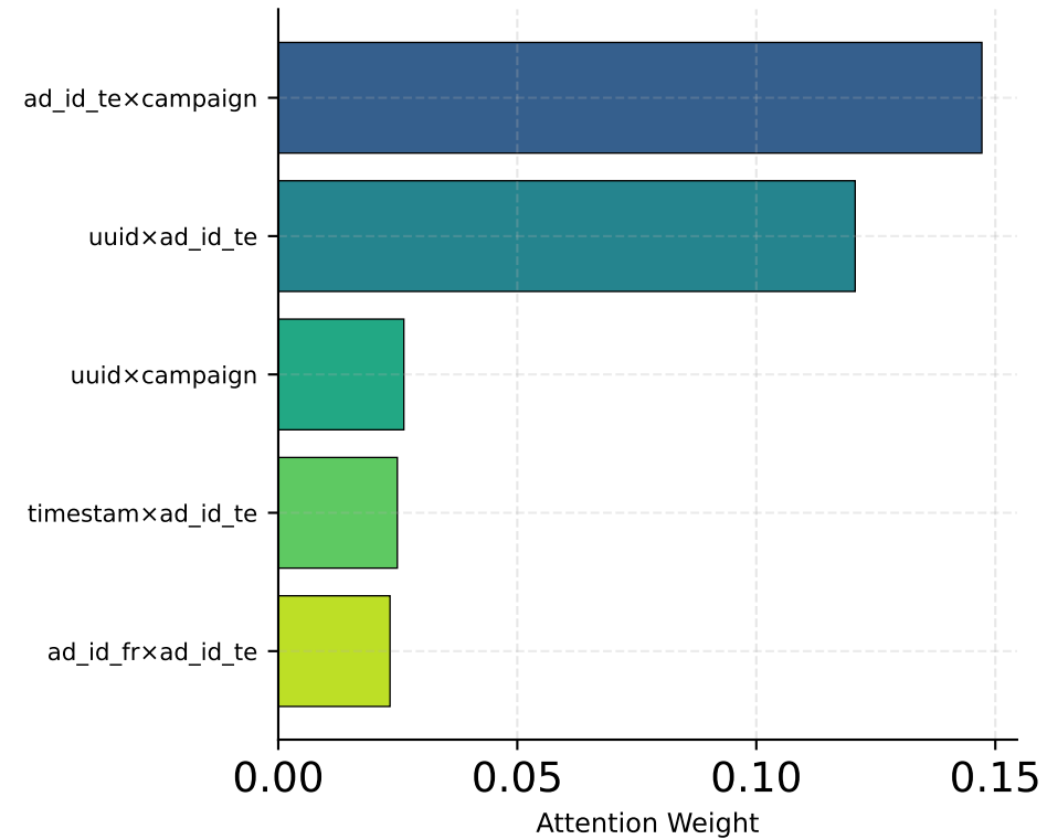
Outbrain
