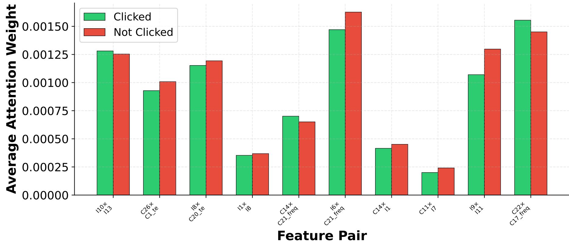
Criteo: Attention Weights by Click Status (Top-10)
