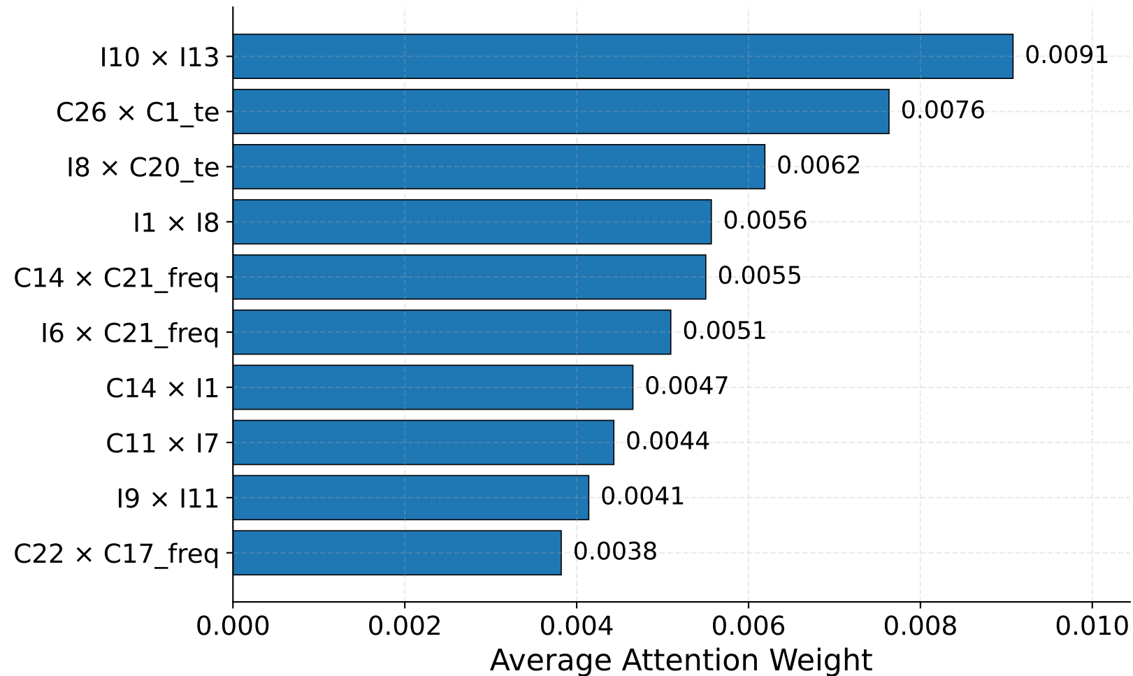
Criteo: Top-10 Feature Interactions
