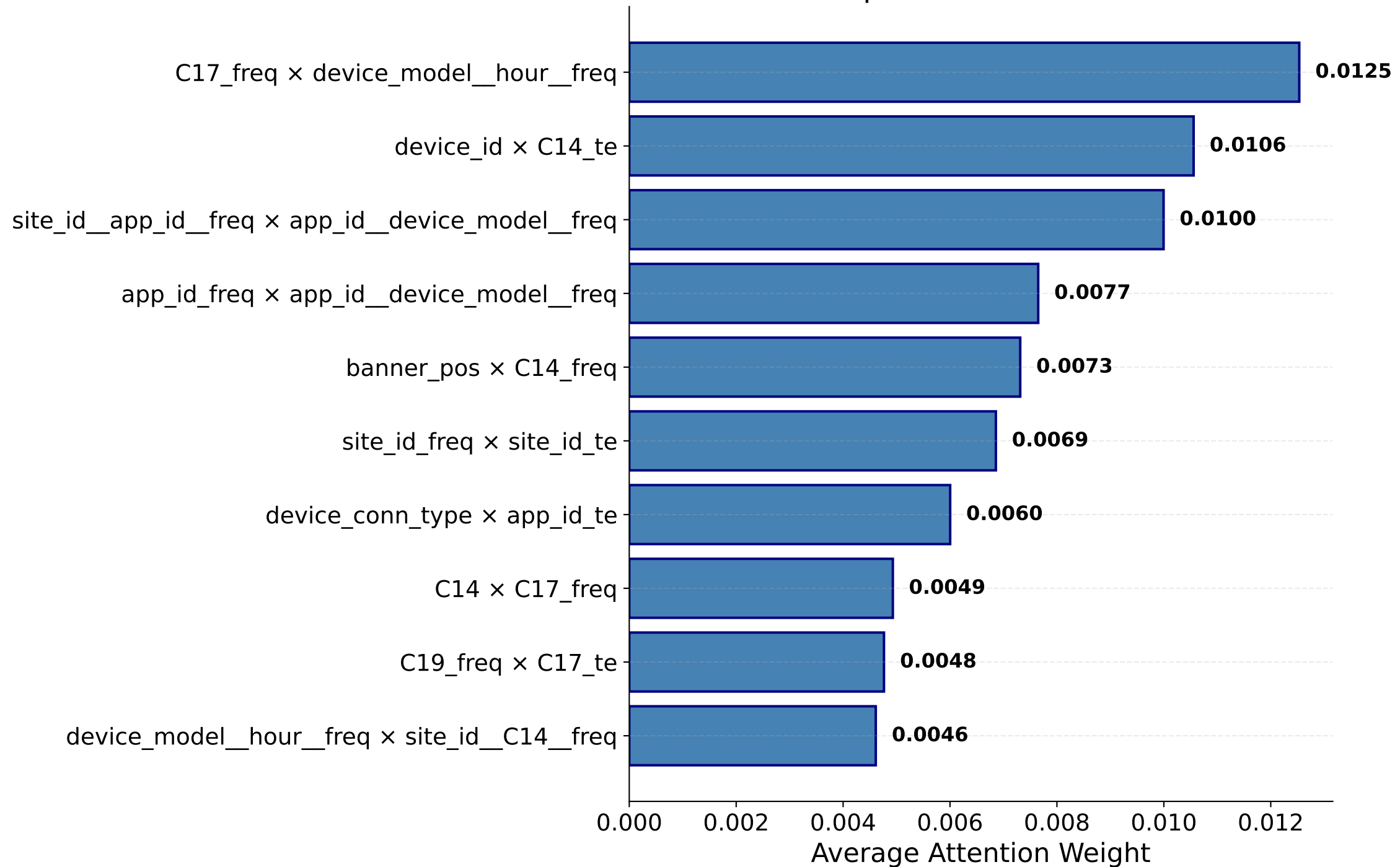
Avazu: Top-10 Feature Interactions
