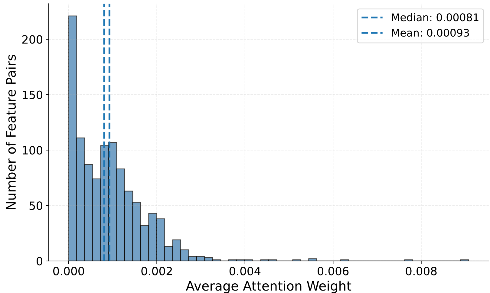
Criteo: Distribution of Attention Weights
