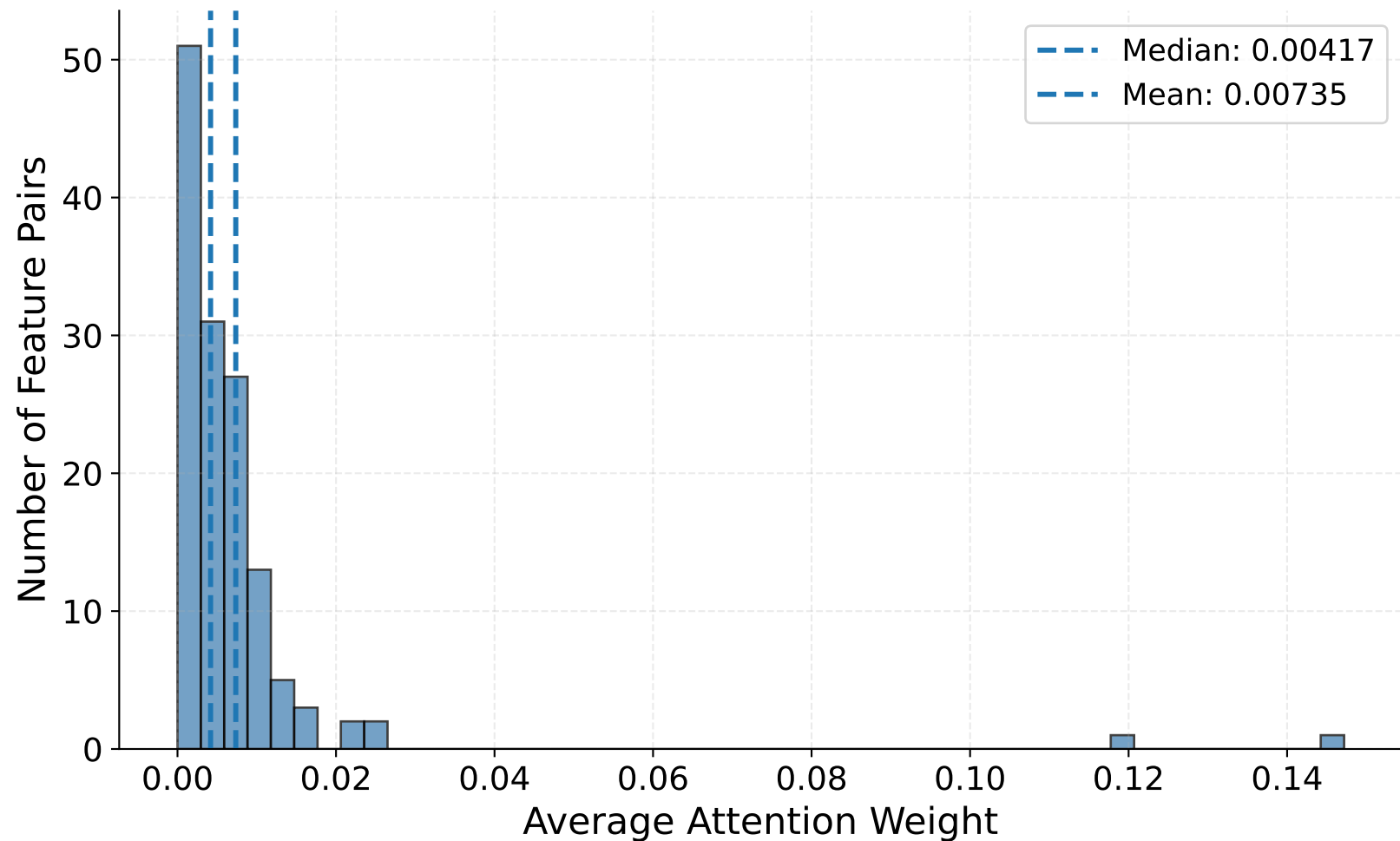
Outbrain: Distribution of Attention Weights
