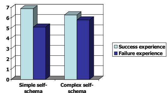
Linville's study (1987)
