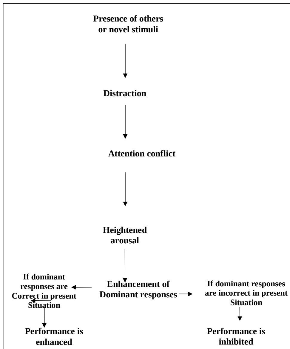
Distraction-conflict theory
