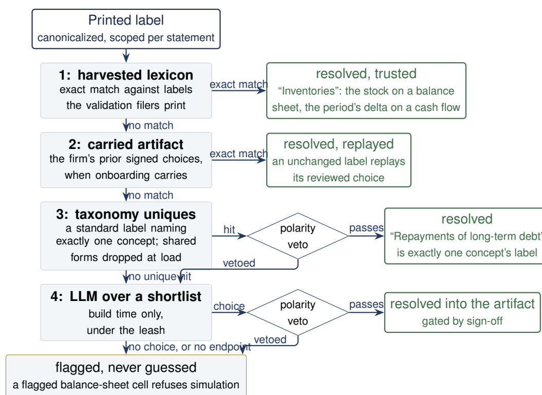
Figure 4. The mapping ladder as a decision flow, with the worked cases from the text embedded at each rung. The two exact-match rungs are trusted; the two heuristic rungs pass the balance-polarity veto, and a veto at the taxonomy tier falls through to the LLM rather than flagging. The LLM runs at build time only, its choices land in the mapping artifact, and sign-off gates them; anything that survives no rung is flagged, never guessed, and a flagged balance-sheet cell refuses simulation.
