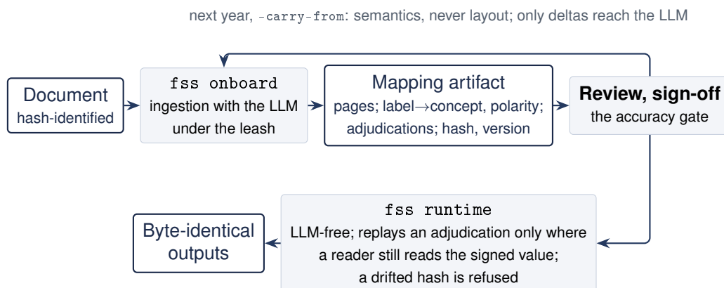
Figure 5. The onboarding lifecycle. fss onboard runs the full ingestion pipeline with the LLM enabled under the leash; every entry in the resulting mapping artifact is a survivor of the mechanical validators, and the artifact binds to the document's hash and carries a sign-off field. fss runtime never constructs an LLM client: it re-extracts deterministically, replays an adjudication only where a deterministic reader still reads the signed value, refuses a drifted hash with re-onboarding required, and reruns byte-identically. A prior year's signed artifact can seed the next year's onboarding: carry seeds semantics, never layout, and only genuine deltas reach the LLM and the reviewer.
