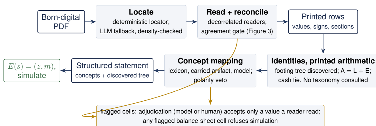
Figure 4. Untagged ingestion validates before it interprets. Printed rows that survive the reader gate are checked arithmetically first: the footing solver discovers the subtotal tree from the numbers themselves, and A = L + E and the cash tie bind on the printed totals, with no taxonomy consulted. Concept mapping then attaches semantics to validated numbers, the encoder stores what survived, and every failure is a flag, never a guess: adjudication can resolve a flag only into a value a deterministic reader read, and a flagged balance-sheet cell refuses simulation.
