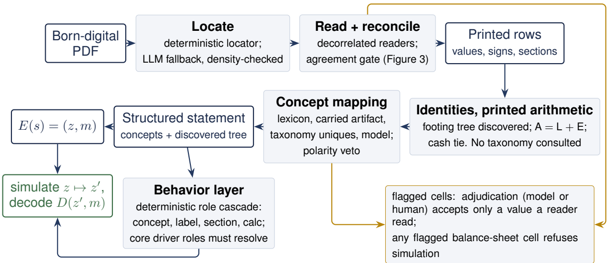
Figure 4. Untagged ingestion validates before it interprets. Printed rows that survive the reader gate are checked arithmetically first: the footing solver discovers the subtotal tree from the numbers themselves, and A = L + E and the cash tie bind on the printed totals, with no taxonomy consulted. Concept mapping then attaches semantics to validated numbers, the encoder stores what survived, and every failure is a flag, never a guess: adjudication can resolve a flag only into a value a deterministic reader read, and a flagged balance-sheet cell refuses simulation. The behavior layer joins at simulation time: the deterministic role cascade classifies every mapped line, and those roles are what the engine and the driver layer consume to advance the state; the identities and the encoding need nothing from them, and a firm whose core driver roles do not resolve is refused simulation with the missing roles named.
