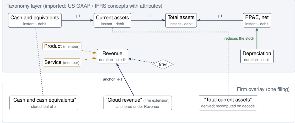
Figure 2. The state space as a typed graph, drawn on a fragment of the validation build’s overlays. Nodes are taxonomy concepts carrying the attributes the simulator relies on: period type (instant = stock, duration = flow) and balance polarity. Solid navy arrows are composition edges imported from the filing’s calculation linkbases, with their weights; dashed gold arrows are dimensional aggregation (Apple discloses product and service revenue members on the statement face); the heavy green arrow is an authored law of motion (depreciation drains the capital stock); the dash-dotted arrow is a driver attachment from Section 8; dotted slate lines show native lines resolving onto nodes through the imported label and synonym index. The overlay beneath shows the three resolution cases from the text: a native line stored as a leaf of z , a firm extension anchored into the calculation subtree (SAP’s cloud revenue under IFRS revenue), and a derived subtotal recomputed on decode.
