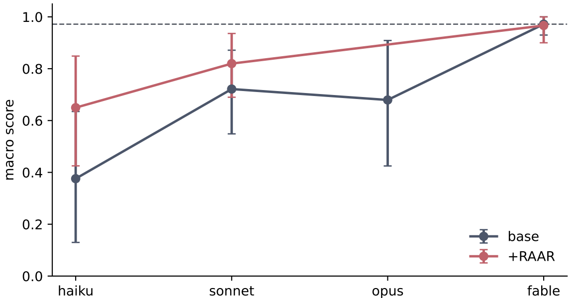
Macro quality across the model ladder
