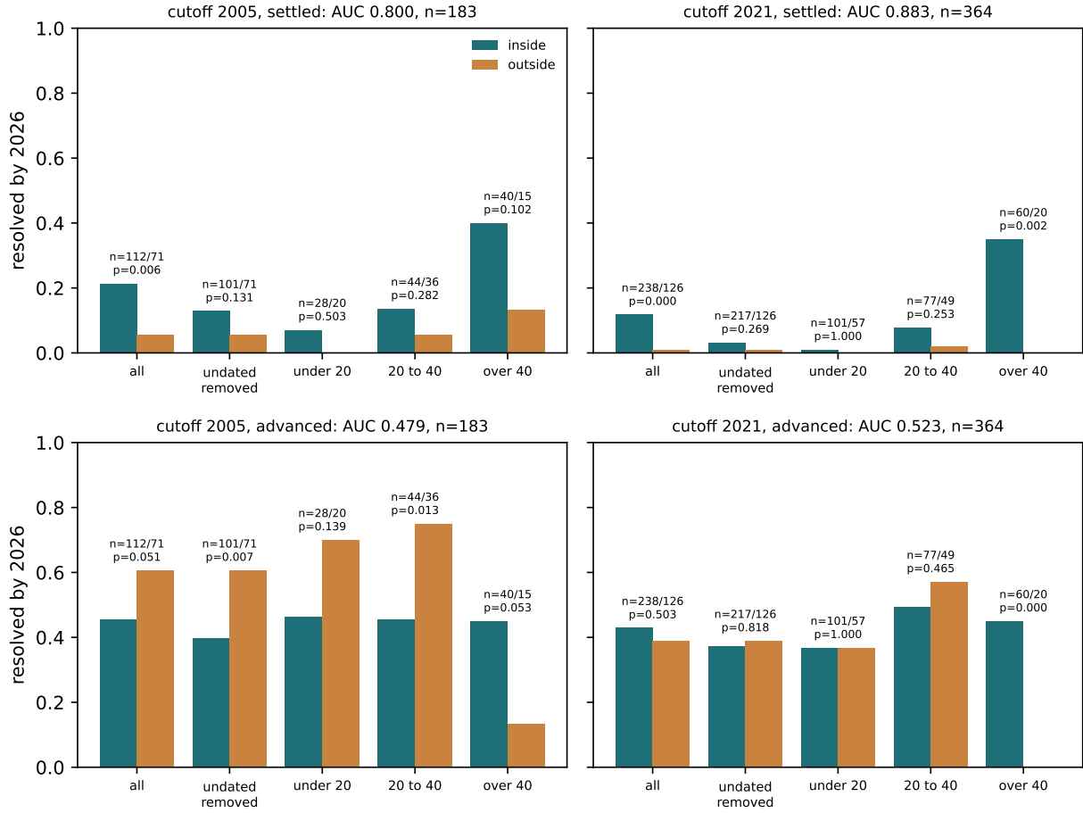
Figure 2: Resolved rate by 2026 inside and outside the cutoff frontier under both codings, over all scored rows, with the undated solved rows removed, and by length band [empirical: output/solvability-frontier/report/backtest.json, 2026-10-06, npx ts-node scripts/build-solvability-frontier-report.ts].
