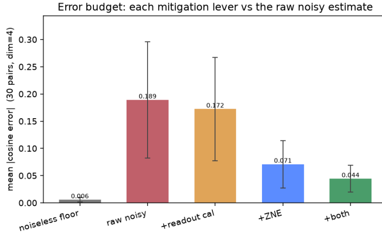
Figure 4: Error budget: noiseless floor \rightarrow raw \rightarrow readout \rightarrow ZNE \rightarrow both, on the Hadamard test.
