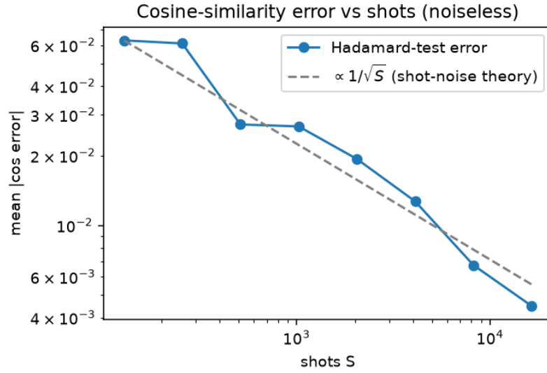
Figure 2: Cosine-similarity error vs shots — follows the 1/\sqrt{S} shot-noise law.
