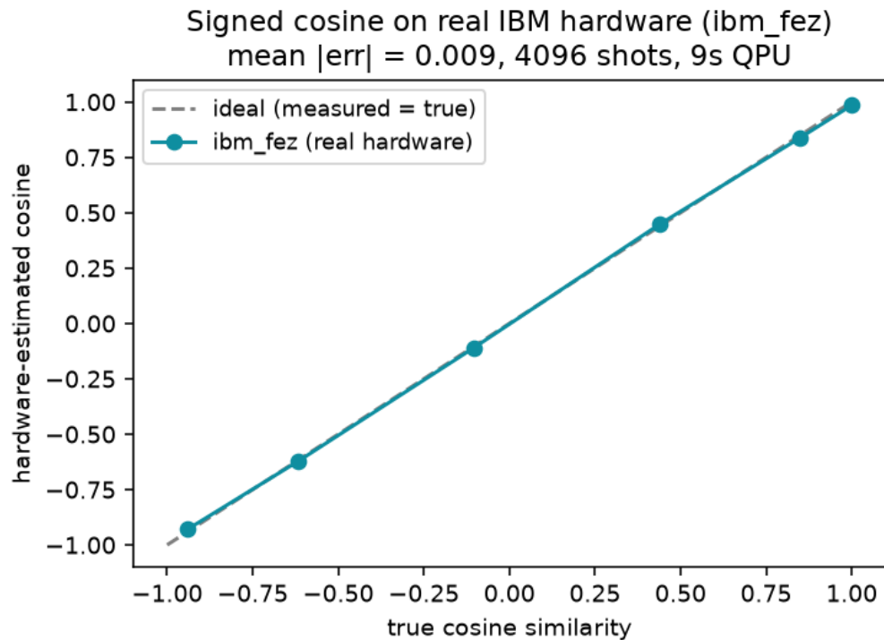
Figure 1: Signed cosine measured on real IBM hardware vs the true value — mean error 0.009 across the full range.
