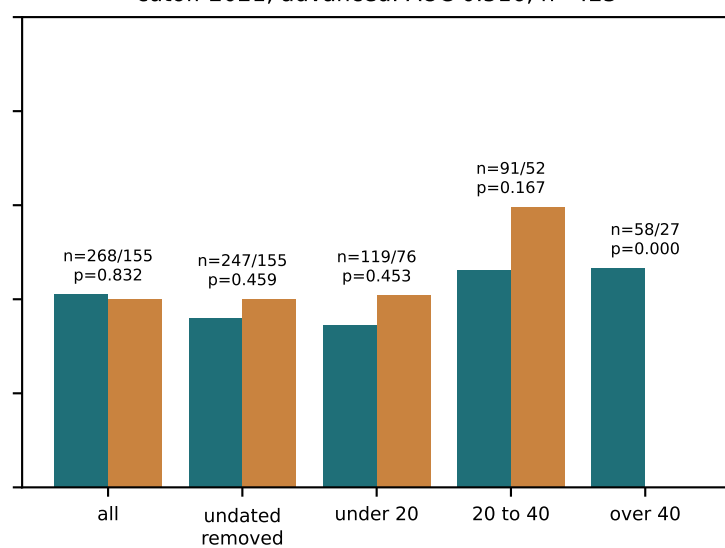
cutoff 2021, advanced: AUC 0.516, n=423
