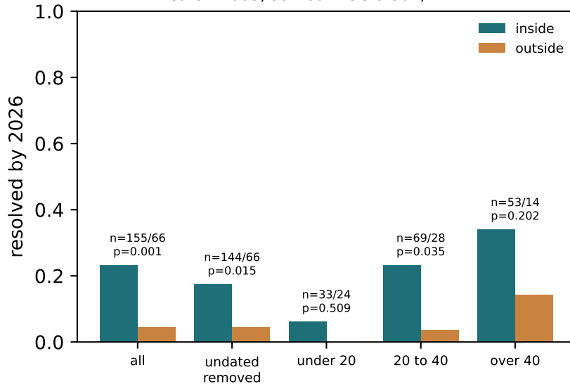
cutoff 2005, settled: AUC 0.807, n=221
