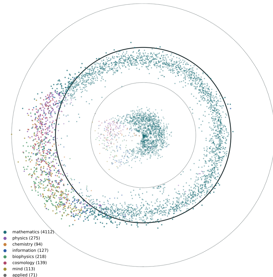
Figure 2: The frontier on 5,149 rows. Solved rows fill the inner disc by reach, open rows inside fill the ring up to the circle at 0.759, outside rows sit beyond it by how far their reach falls short, and any unsampled rows would be grey crosses [empirical: output/solvability-frontier/report/frontier.json , 2026-10-08, npx ts-node scripts/build-solvability-frontier-report.ts ].
