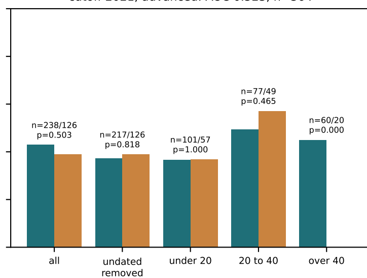
cutoff 2021, advanced: AUC 0.523, n=364
