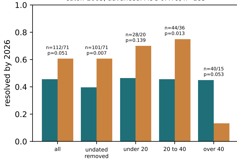
cutoff 2005, advanced: AUC 0.479, n=183
