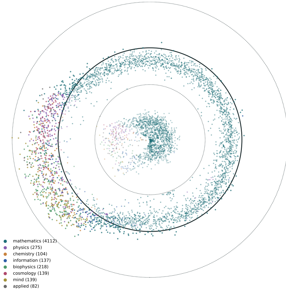
Figure 2: The frontier on 5,206 rows. Solved rows fill the inner disc by reach, open rows inside fill the ring up to the circle at 0.759, outside rows sit beyond it by how far their reach falls short, and any unsampled rows would be grey crosses [empirical: output/solvability-frontier/report/frontier.json , 2026-10-08, npx ts-node scripts/build-solvability-frontier-report.ts ].
