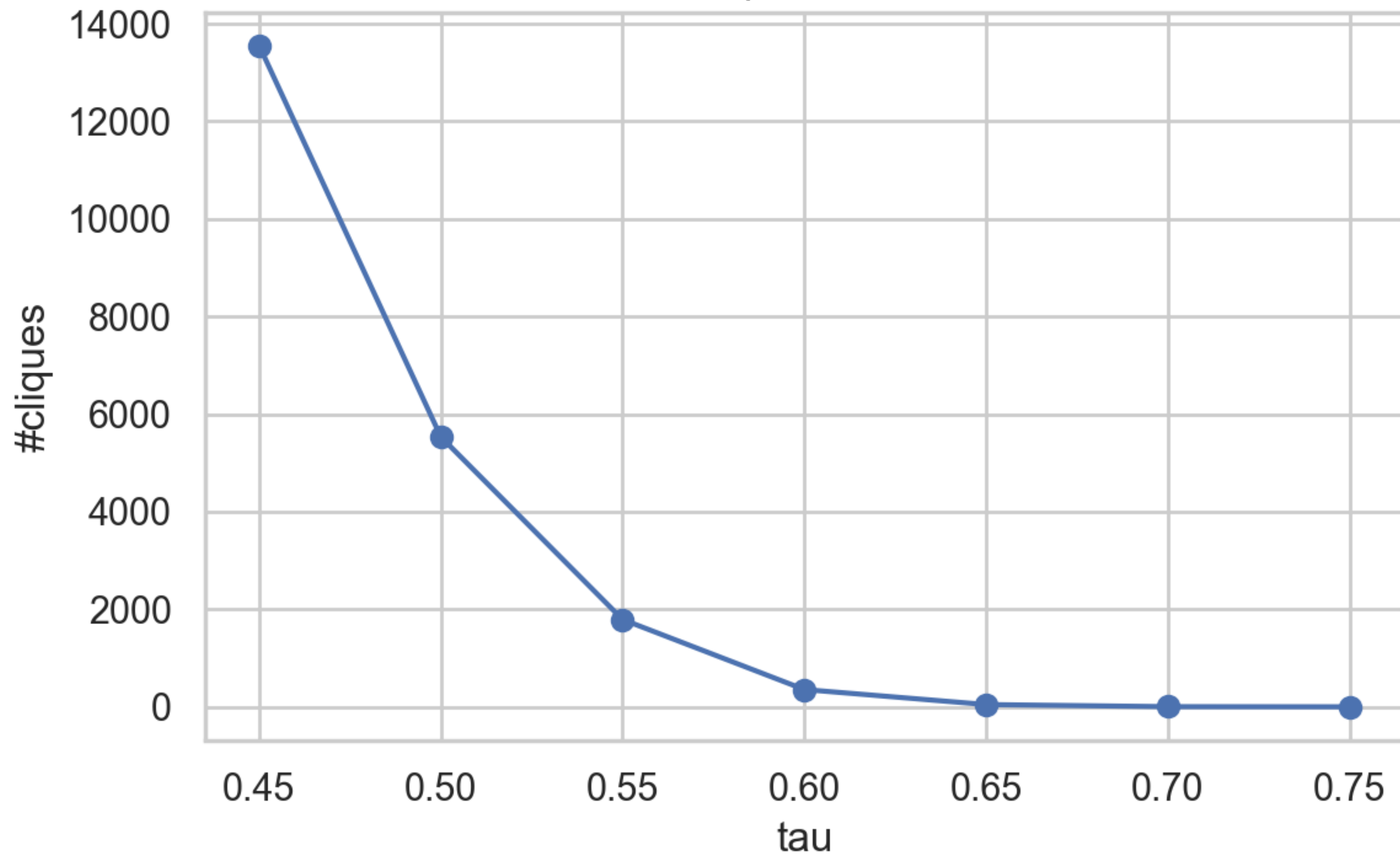
#cliques vs tau
