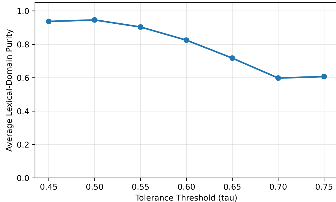
TRANSE: Lexical-Domain Purity vs tau
