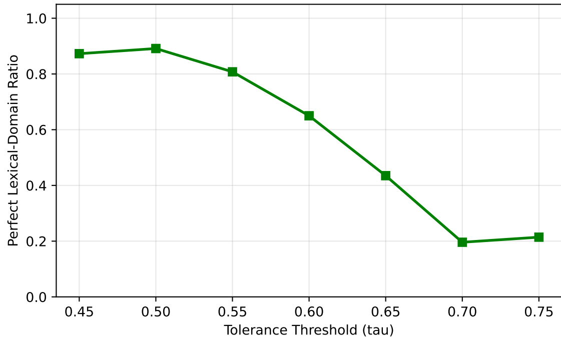
TRANSE: Perfect Domain Ratio vs tau
