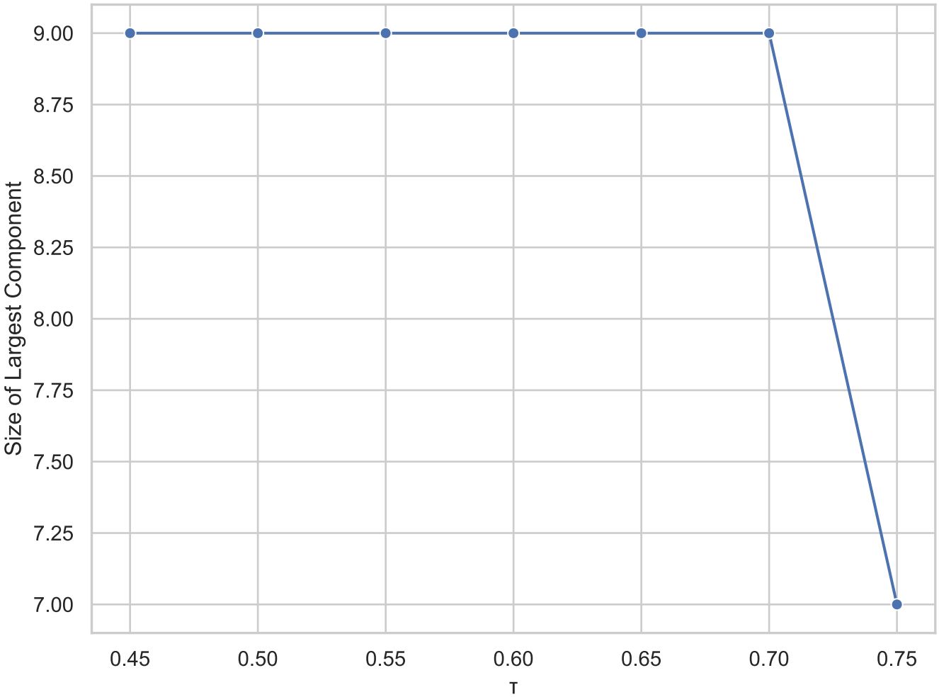
Size of Largest Component vs \tau
