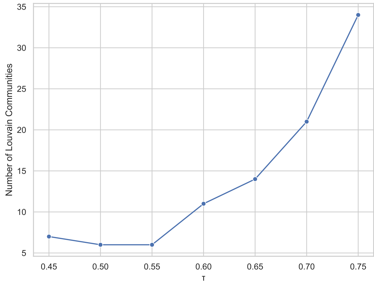
Number of Louvain Communities vs \tau
