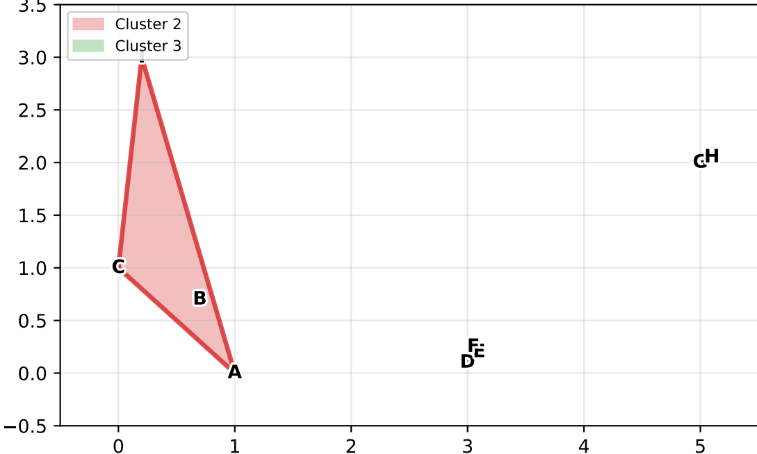
K-Means Partition (Hard Assignment)
