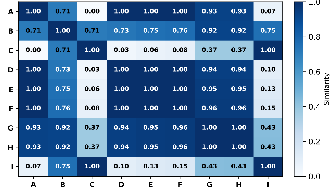
Cosine Similarity Matrix
