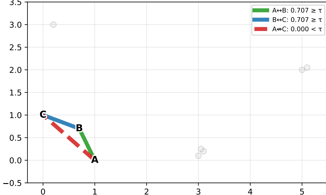
Non-Transitivity Demo ( \tau=0.70 ) A \sim B , B \sim C , but A \not\sim C
