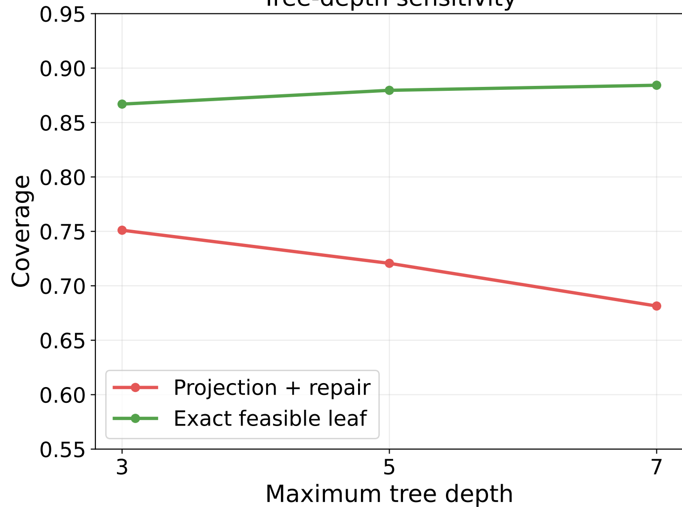
Tree-depth sensitivity
