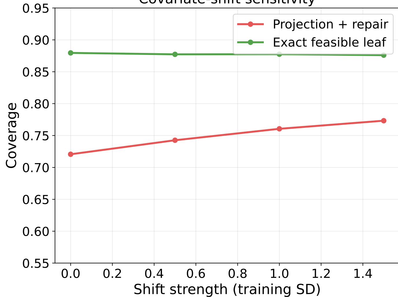
Covariate-shift sensitivity
