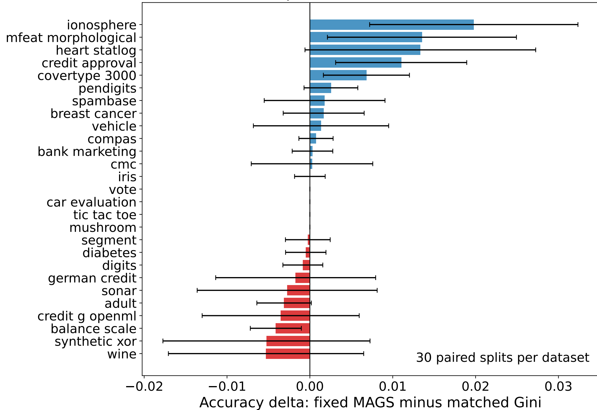
Matched-depth effect at Gaussian noise \sigma = 0.2
