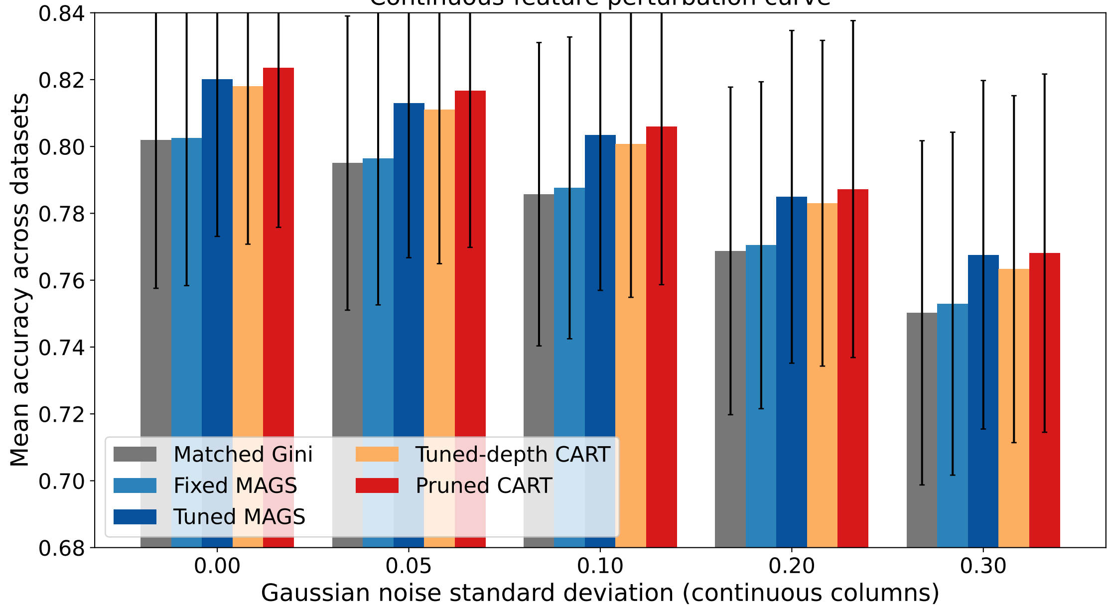
Continuous-feature perturbation curve
