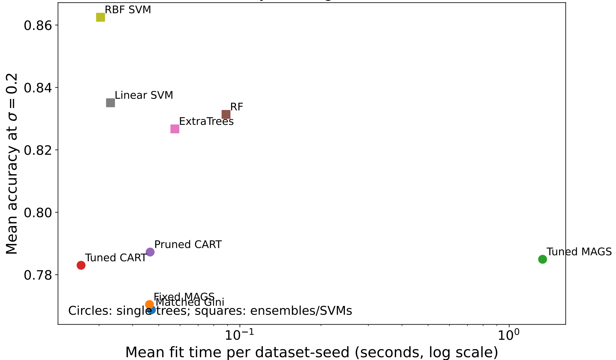
Predictive accuracy, training time, and model class
