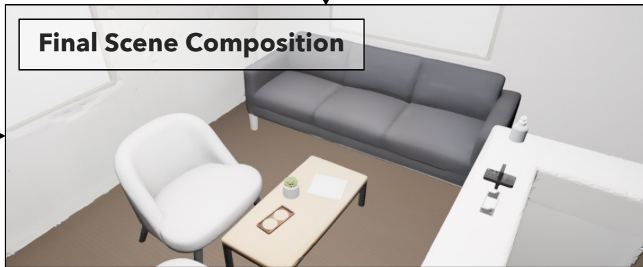
FIRE3D-Shape Network
