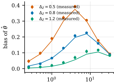
(a) bias is hump-shaped; line = law with \hat{v}
