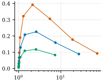
(b) bias vs conditioning: not monotone
