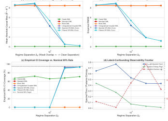
Figure 3: The Latent-Confounding Difficulty Frontier across 500 Monte Carlo Replications. (a) Absolute causal bias |\hat{\theta} - \theta^*| vs. regime separation \Delta_Z . In this benchmark DGP, Standard and Block DML exhibit approximately constant omitted-regime bias across \Delta_Z ; OR-DML bias contracts smoothly as separation increases. (b) Empirical RMSE. (c) Empirical 95% CI coverage vs. nominal 95% target. (d) Factorial plane: Absolute bias |\hat{\theta} - \theta^*| across the joint (\bar{\epsilon}_\gamma, \lambda_{\min}(\mathbf{J})) frontier, decoupling proxy difficulty from causal overlap.
