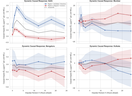
Figure 4: Dynamic Exposure-Response Curves \hat{\theta}_h across Horizons h \in [0, 24] Hours for Delhi, Mumbai, Bengaluru, and Kolkata. Shaded bands represent 95% HAC confidence intervals. Regime stratification reveals substantial structural heterogeneity in dynamic pollutant accumulation over multi-hour horizons.
