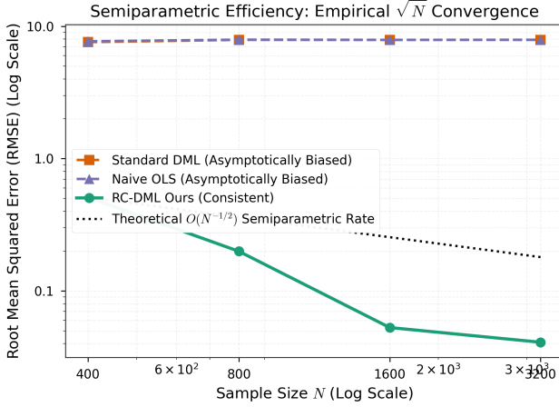
Figure 3: Semiparametric Efficiency: Empirical \sqrt{N} Convergence. Log-log scaling of RMSE vs. sample size N \in [400, 3200] . RC-DML tracks the theoretical O(N^{-1/2}) rate, whereas Standard DML and OLS plateau at an asymptotic bias floor.
