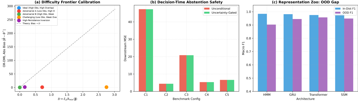
Figure 5: Universal LatentRegimeBench Evaluation. (a) Calibration of causal estimation bias against theoretical degradation ratio \mathcal{D} = \bar{\epsilon}_\gamma / \lambda_{\min}(\mathbf{J}) . (b) Decision-time abstention safety comparing unconstrained point MSE against uncertainty-gated MSE. (c) Representation zoo out-of-distribution (OOD) generalization across HMM, GRU, Causal Transformer, and Linear SSM.
