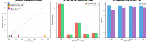
Figure 5: Universal LatentRegimeBench Evaluation. (a) Calibration of causal estimation bias against theoretical degradation ratio \mathcal{D} = \bar{\epsilon}_{\gamma} / \lambda_{\min}(\mathbf{J}) . (b) Decision-time abstention safety comparing unconstrained point MSE against uncertainty-gated MSE. (c) Representation zoo out-of-distribution (OOD) generalization across HMM, GRU, Causal Transformer, and Linear SSM.
