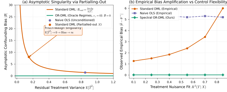
Figure 2: Visualizing the Frisch-Waugh Singularity and Omitted Regime Bias. (a) As residual treatment variance \mathbb{E}[T_t^2] \rightarrow 0 via partialling-out X_t , omitted regime bias \mathcal{B}_{\text{confounding}} explodes hyperbolically in Standard DML, while OR-DML (Oracle Regimes, \varepsilon_\gamma = 0 ) remains strictly unbiased ( \mathcal{B} = 0 ). (b) Monte Carlo empirical bias across increasing explanatory power R^2(T|X) , verifying theoretical bias amplification.
