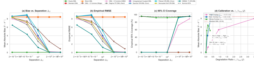
Figure 3: The Latent-Confounding Difficulty Frontier across 500 Monte Carlo Replications. (a) Absolute causal bias |\hat{\theta} - \theta^*| vs. regime separation \Delta_Z . (b) Empirical RMSE. (c) Empirical 95% CI coverage vs. nominal 95% target. (d) Corrected factorial mechanism test: causal L_2 error vs. \varepsilon_\gamma/\lambda_{\min}(J) across 49 independently controlled cells (100 replications each), where task conditioning is varied through residual treatment innovation variance after regime-aware nuisance residualization.
