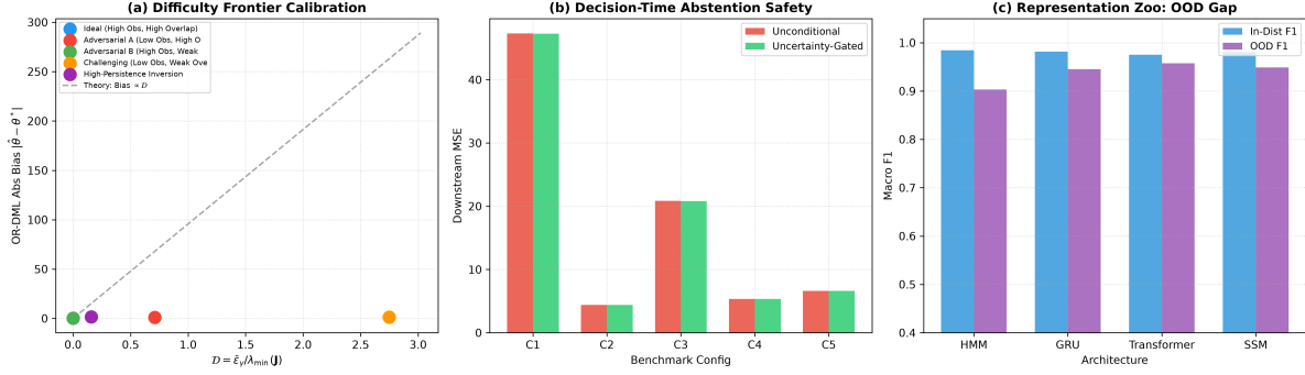
Figure 5: Universal LatentRegimeBench Evaluation. (a) Bias calibration against theoretical degradation ratio \mathcal{D} = \bar{E}_\gamma / \lambda_{\min}(\mathbf{J}) . (b) Decision-time abstention safety comparing unconstrained vs. gated MSE. (c) Representation zoo OOD generalization across HMM, GRU, Transformer, and Linear SSM.
