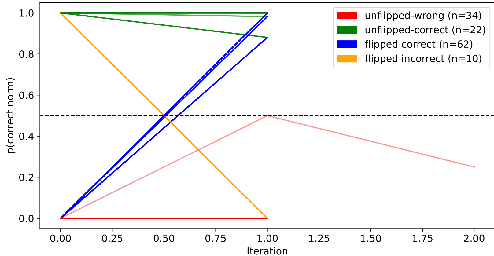
p(correct norm) confidence over iterations (n=128)
