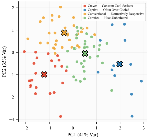
Feature Space Projection (PCA)
