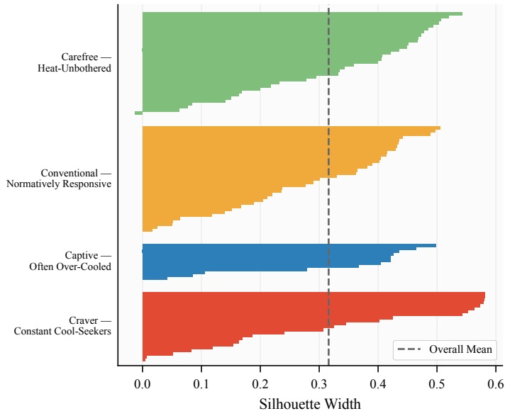
Per-Archetype Silhouette Widths
