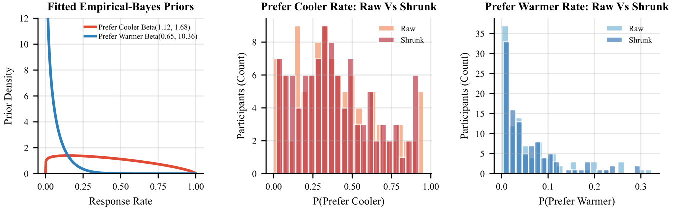
Figure 4: Constructing stable person-level features through empirical-Bayes shrinkage. Fitted Beta priors are shown on the left, and the center and right panels show how participants’ raw prefer-cooler and prefer-warmer rates are pulled toward the cohort mean, most strongly for those with few responses.
