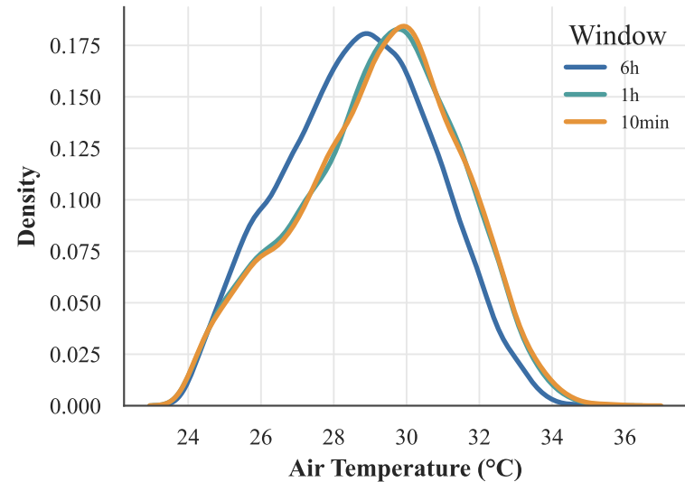
Air Temperature
