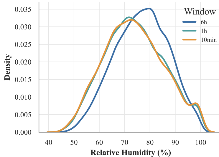
Relative Humidity
