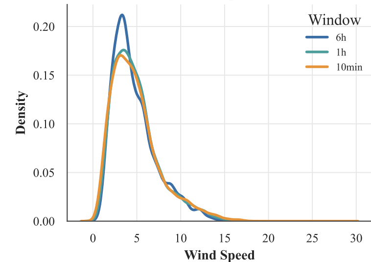
Wind Speed
