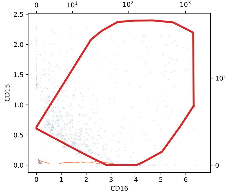
Hierarchy 1
