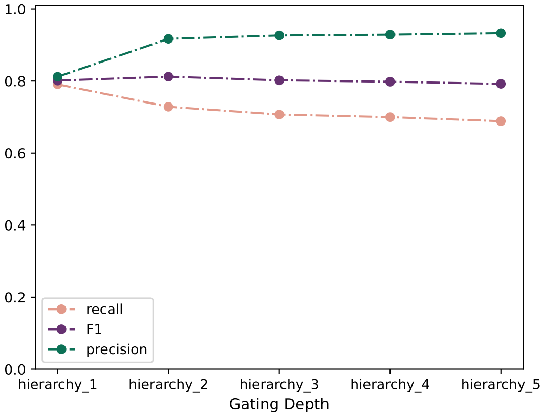
Performance - cluster CD16+ CD8+ T cell
