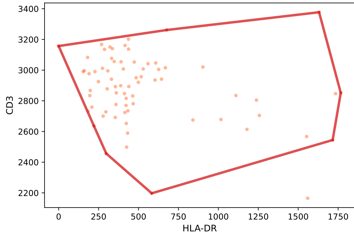
cluster CD16+ CD4+ T cell - hierarchy 5
