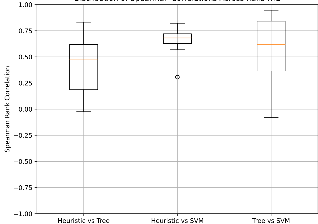
Distribution of Spearman Correlations Across Runs lvl2
