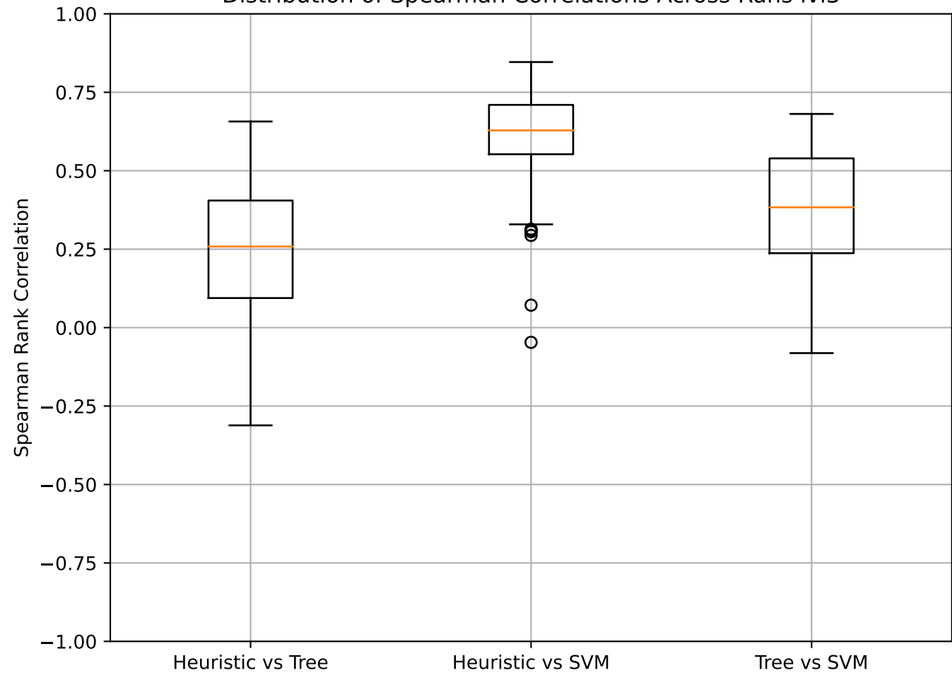
Distribution of Spearman Correlations Across Runs lvl3
