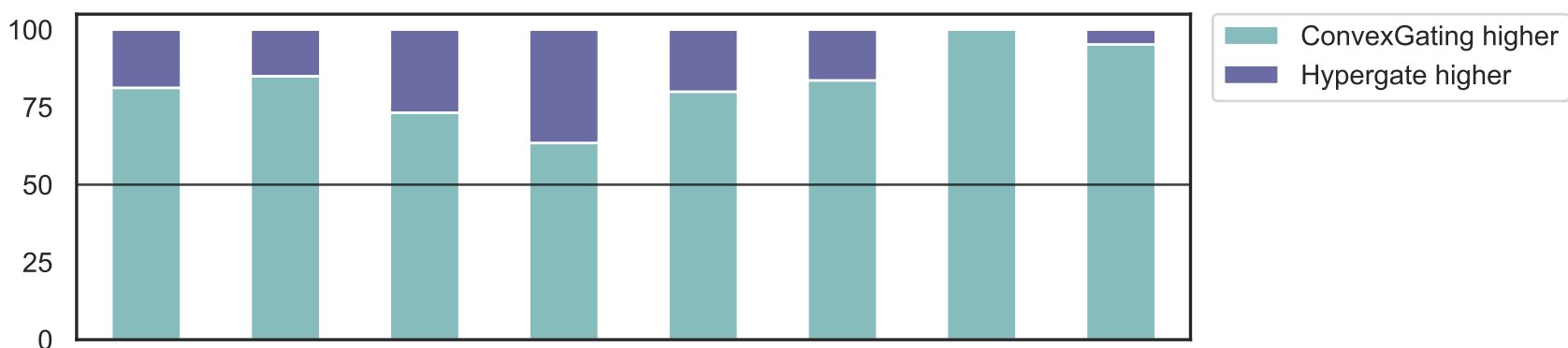
Recall
