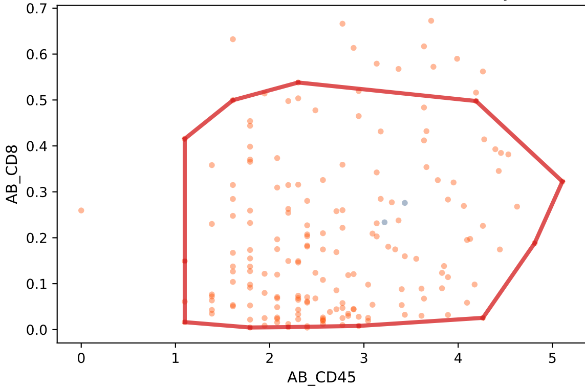
cluster HLA-DR+ CD16+ CD4+ T cell - hierarchy 3
