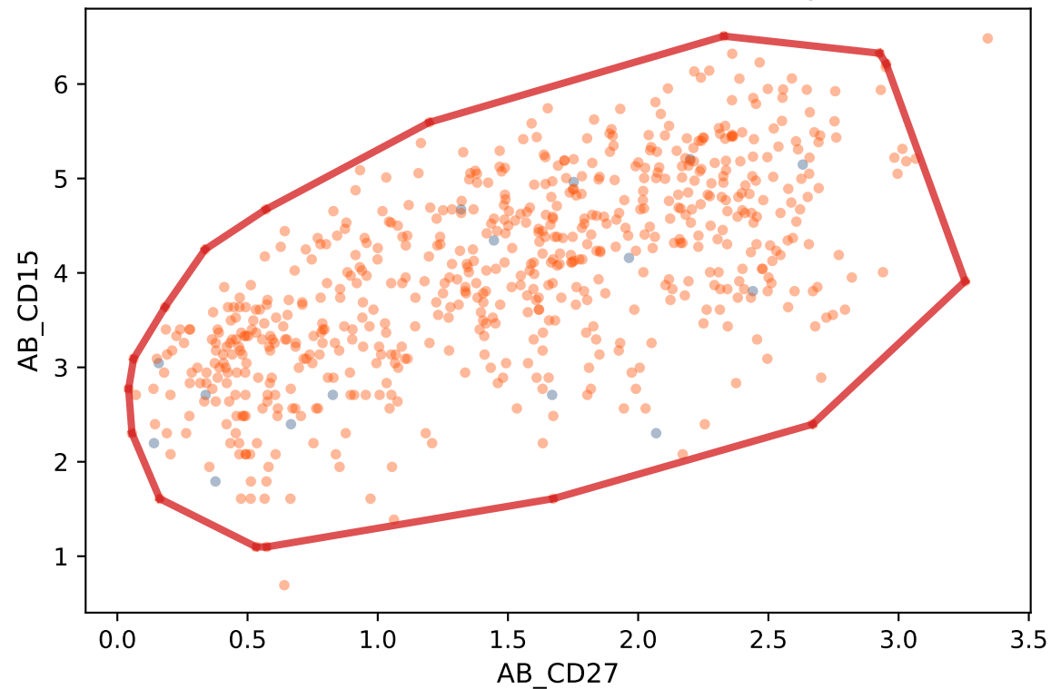
cluster CD16+ CD4+ T cell - hierarchy 5
