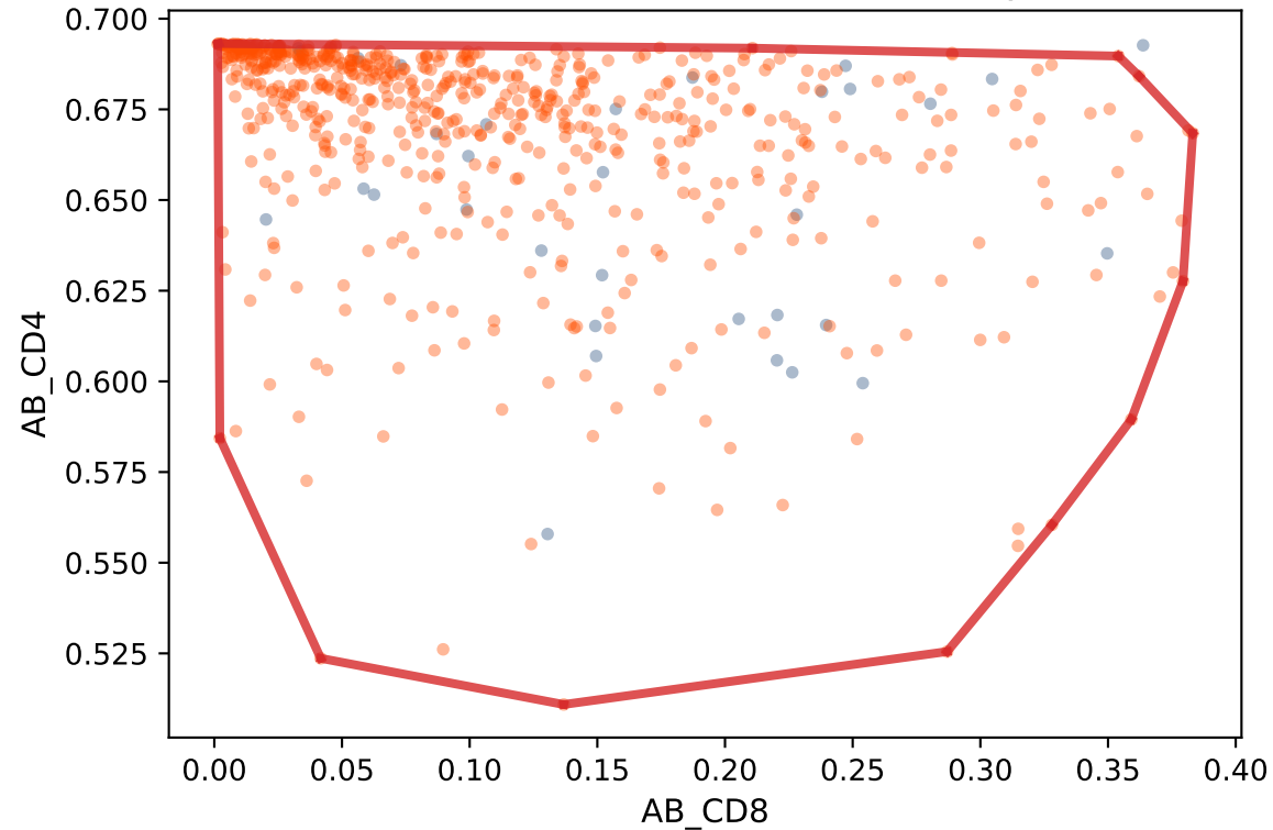
cluster CD16+ CD4+ T cell - hierarchy 4
