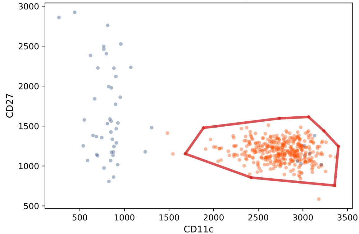
cluster cDC - hierarchy 3
