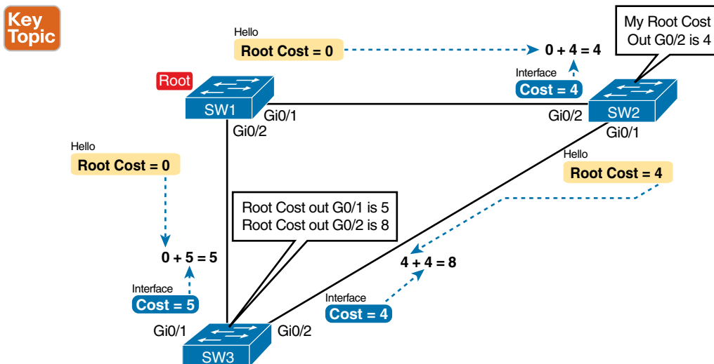
Figure 9-6 How STP/RSTP Actually Calculates the Cost from SW3 to the Root
