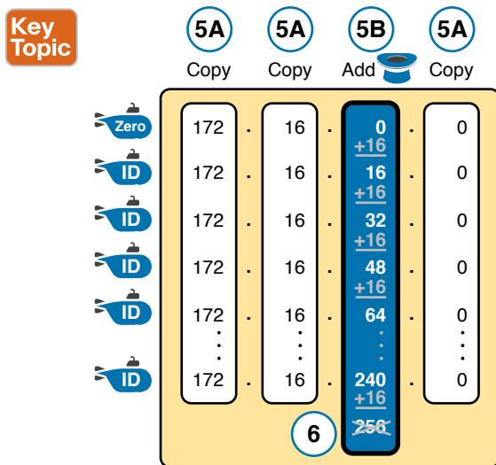
Figure L-9 List of Subnet IDs: 172.16.0.0, 255.255.240.0
