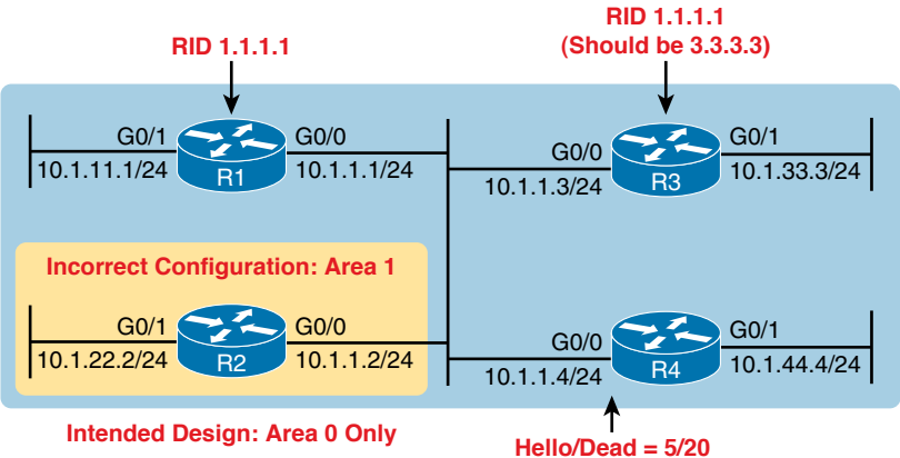
Figure 21-4 Summary of Problems That Prevent OSPF Neighbors on the Central LAN
