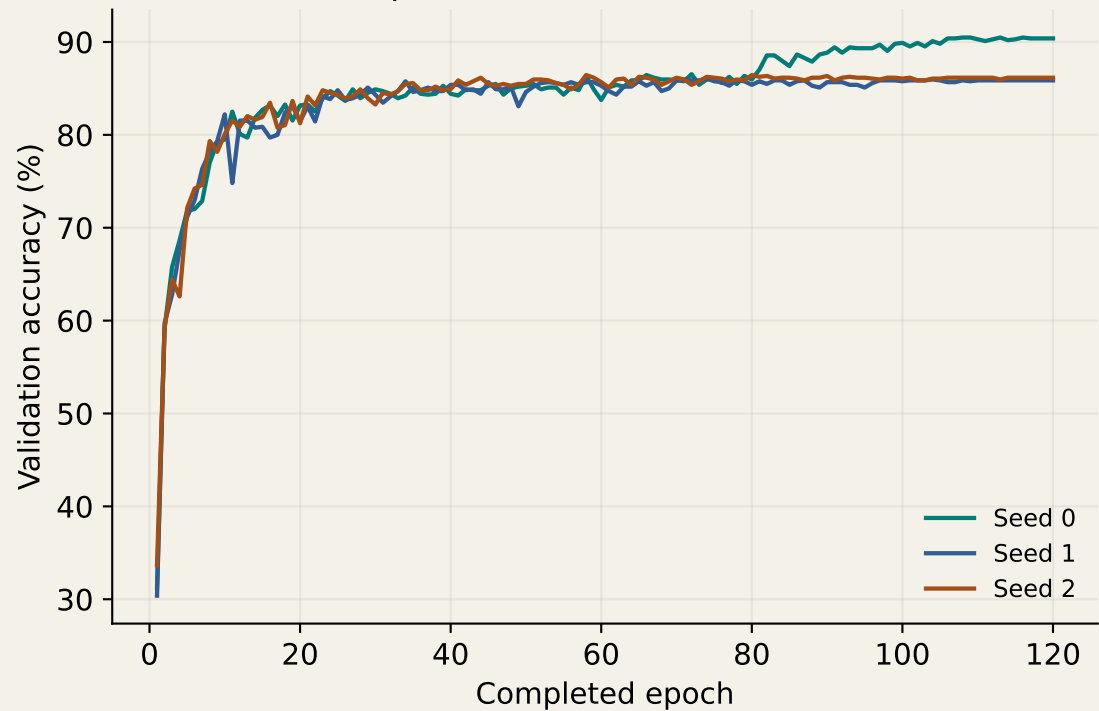
Checkpoint selection uses validation
