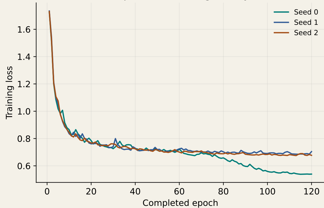
Supervised training history
