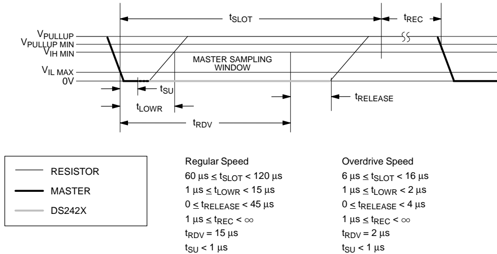
READ/WRITE TIMING DIAGRAM Figure 11 cont'd Read-data Time Slot
