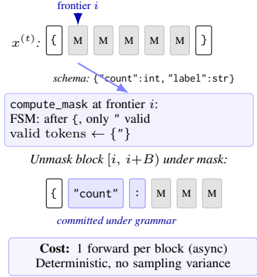
Figure 3: One denoising step under schema {"count":int, "label":str}. LAVE (Zhang et al., 2026) (left) samples K random completions at each frontier token, accepting it only when \geq 1 suffix is valid—stochastic and K\times more expensive per token, hitting the 120 s per-instance timeout on hard schemas. Dgrammar (right) runs compute_mask on the incremental FSM state and unmask an entire block under that mask in one forward pass, overlapped with the next mask computation; the result is deterministic.
