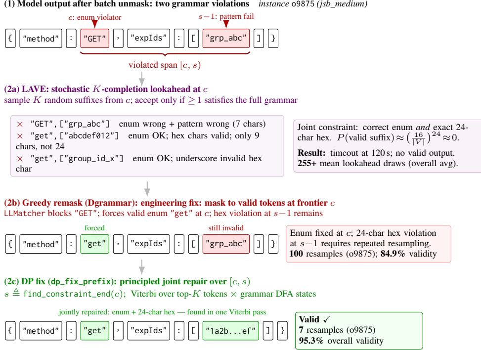
Figure 1: Motivating example from JSONSchemaBench medium instance o9875 (API route config). The schema requires \text{method} \in [\text{"get"}, \text{"post"}, \text{"put"}, \dots] (lowercase enum) and each \text{experienceGroupIds} item to match ^{\wedge}[\text{A-Fa-f0-9}]\{24\}\$ (24-character hex, e.g. MongoDB ObjectId). (1) The diffusion model’s batch unmask produces "GET" (fails lowercase enum, position c ) and "grp_abc" (fails 24-char hex pattern, position s-1 ); the violated span covers both. (2a) LAVE samples K random completions from c : satisfying both the enum and the exact-24 hex pattern simultaneously requires P \approx (16/|V|)^{24} \approx 0 , no valid completion is ever drawn; LAVE times out at 120 s (255+ mean draws overall). (2b) Dgrammar forces "get" at c via LLMatcher masking (enum fixed), but the hex-pattern violation at s-1 requires 100 resamples to generate a valid 24-character string (84.9% overall validity). (2c) DPGrammar runs Viterbi over [c, s) jointly, assigning both "get" and a valid 24-char hex ID in one pass, only 7 resamples on this instance (95.3% overall validity).
