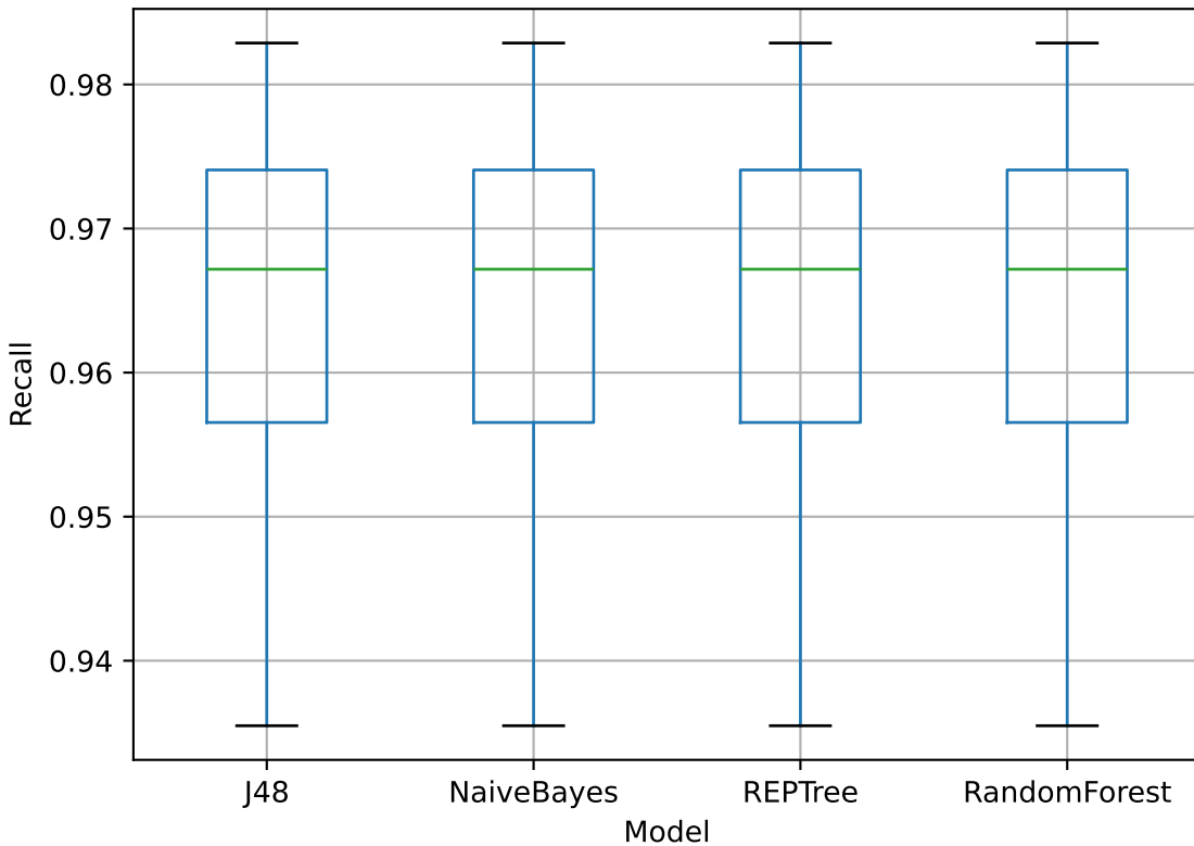
Box and Whisker Plot for Recall
