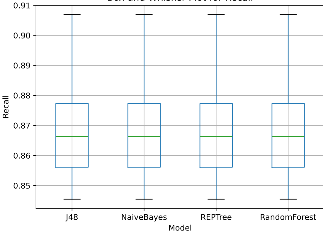
Box and Whisker Plot for Recall
