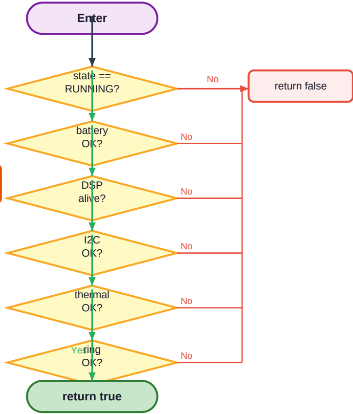
SAFETY_CheckSystem() Flowchart
