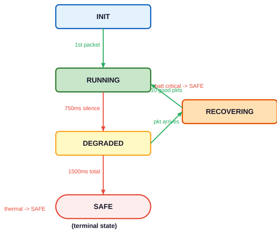
Radio State Machine
