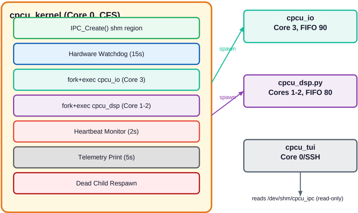
cpcu_kernel Block Diagram
