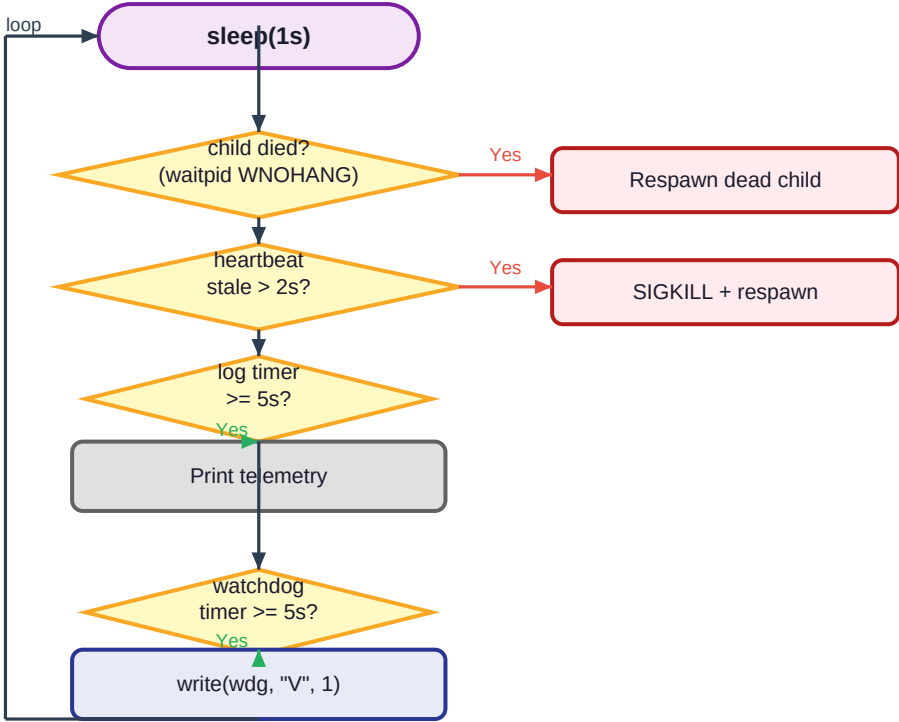
Supervisor Monitor Loop Flowchart
