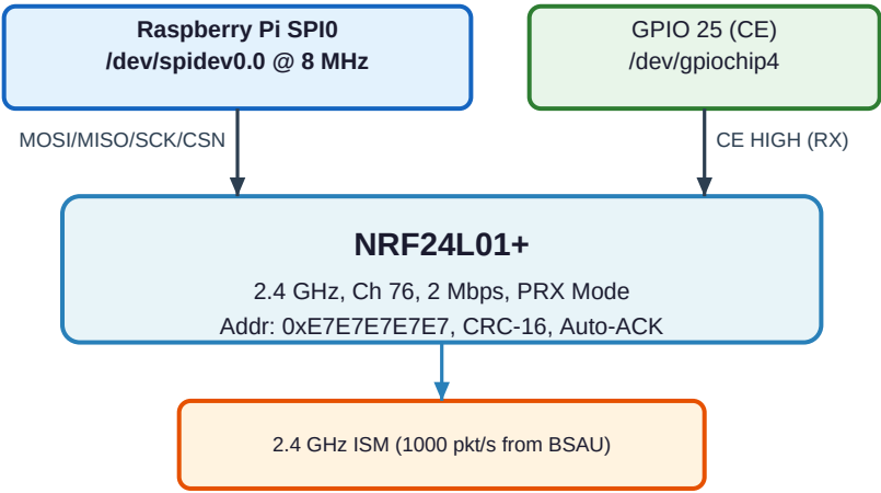
NRF24L01+ SPI Driver Block Diagram
