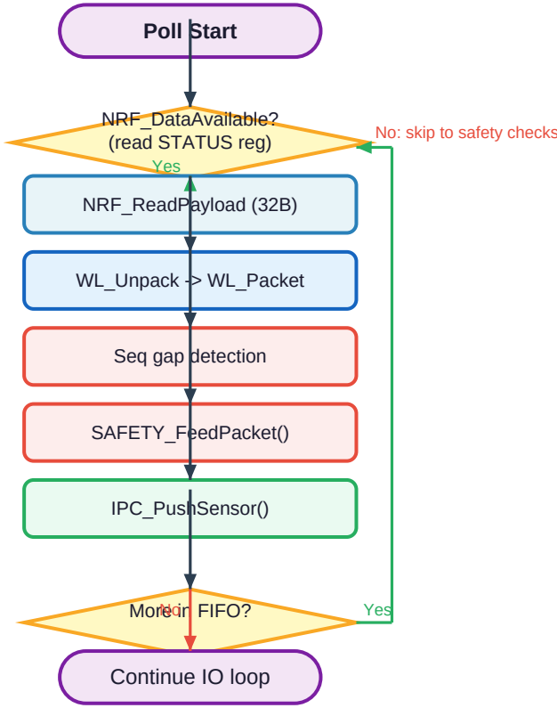
NRF Receive Loop (in cpcu_io)
