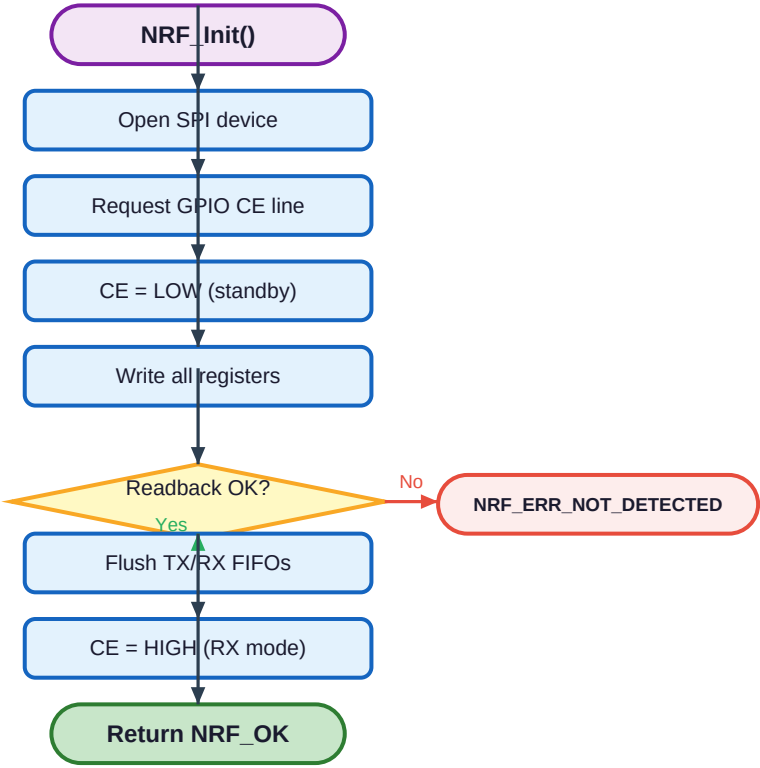
NRF_Init() Flowchart
